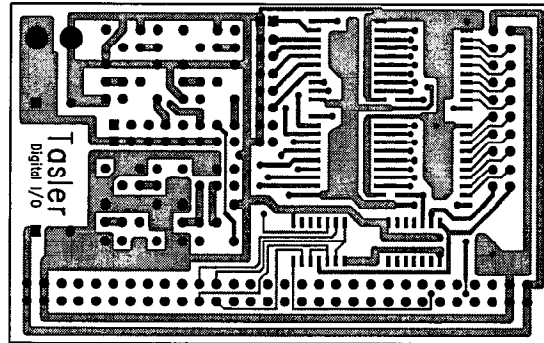
Figure C.4.1: PCB Layout of PIO (Component side)
