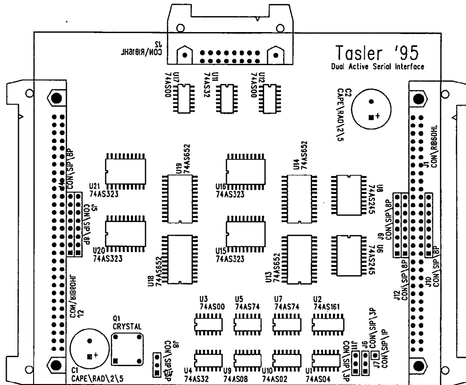
Figure C.2.3: PCB Layout of DASI (Components)
