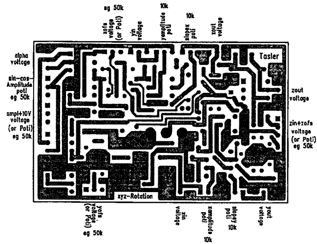
Figure C.7.1: PCB Layout of Coordinate Rotation (Component side)
