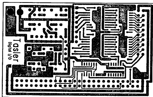
Figure C.4.1: PCB Layout of PIO (Component side)
