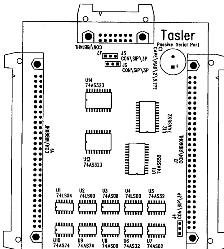
Figure C.3.3: PCB Layout of PSP (Components)
