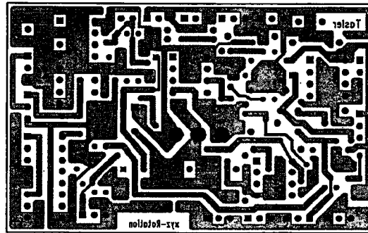
Figure C.7.2: PCB Layout of Coordinate Rotation (Solder side)
