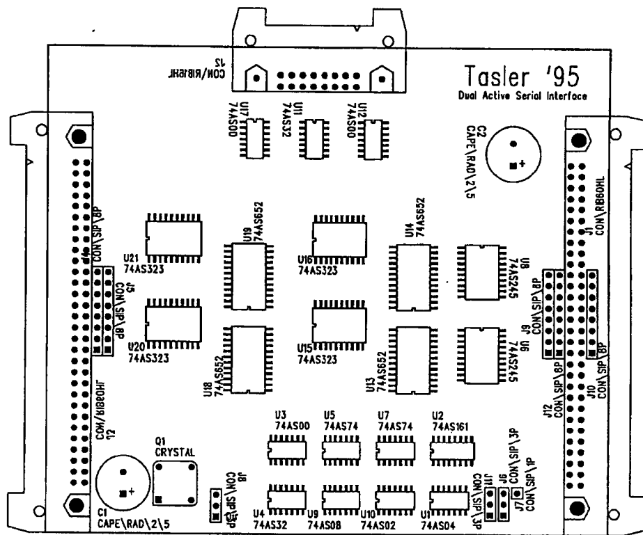
Figure C.2.3: PCB Layout of DASI (Components)
