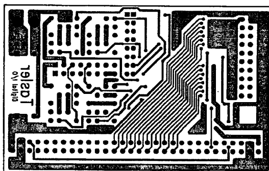
Figure C.4.2: PCB Layout of PIO (Solder side)
