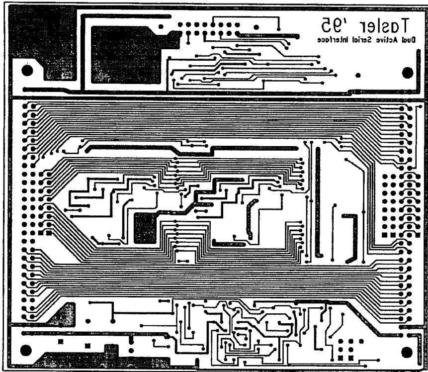
Figure C.2.2: PCB Layout of DASI (Solder side)
