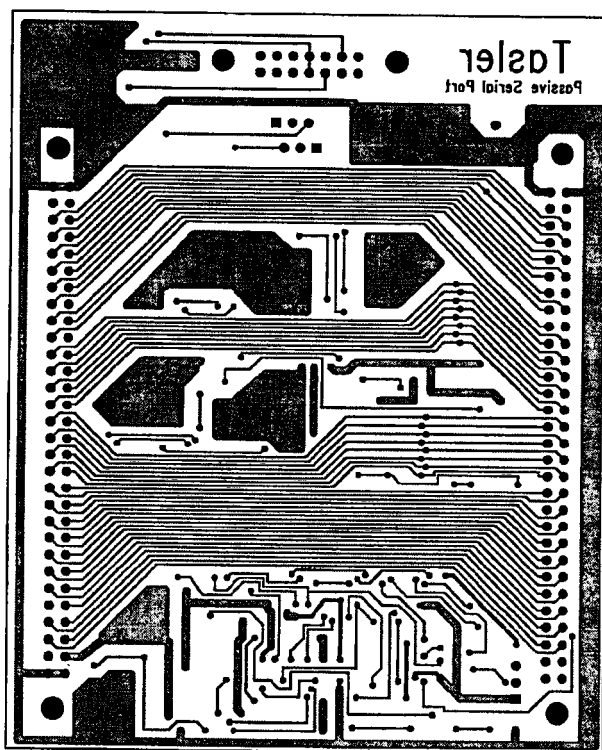
Figure C.3.2: PCB Layout of PSP (Solder side)
