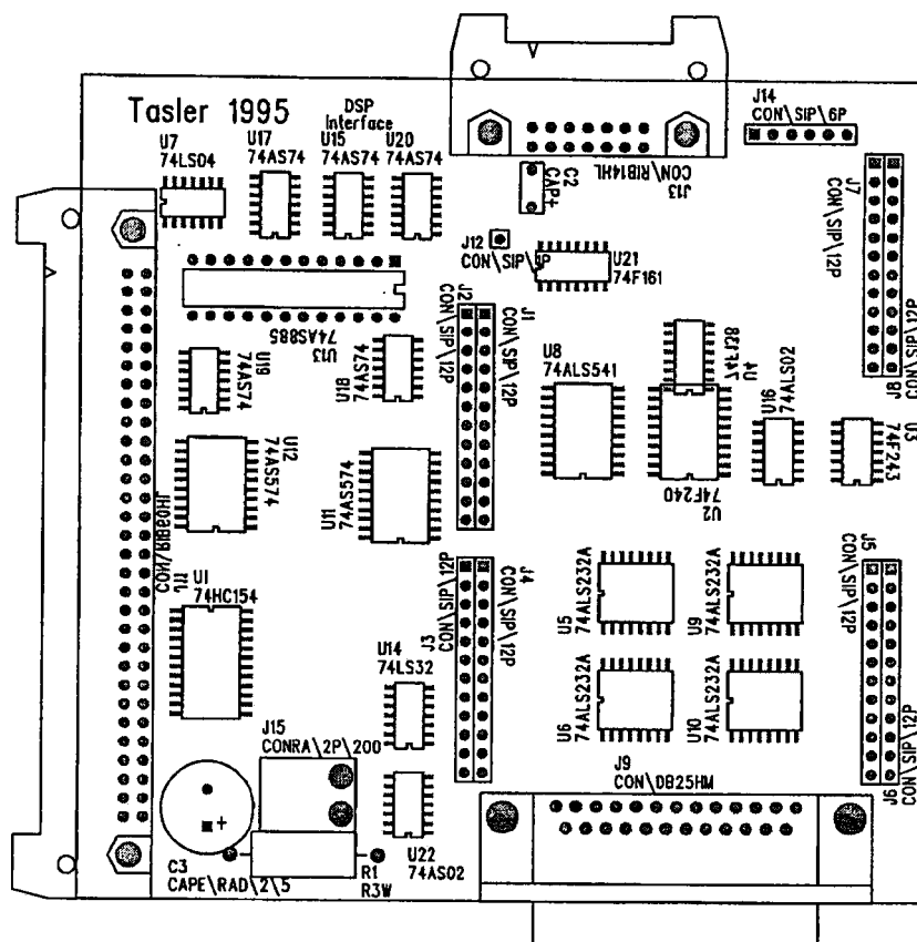
Figure C.1.3: PCB Layout of the DSP Motherboard (Components)
